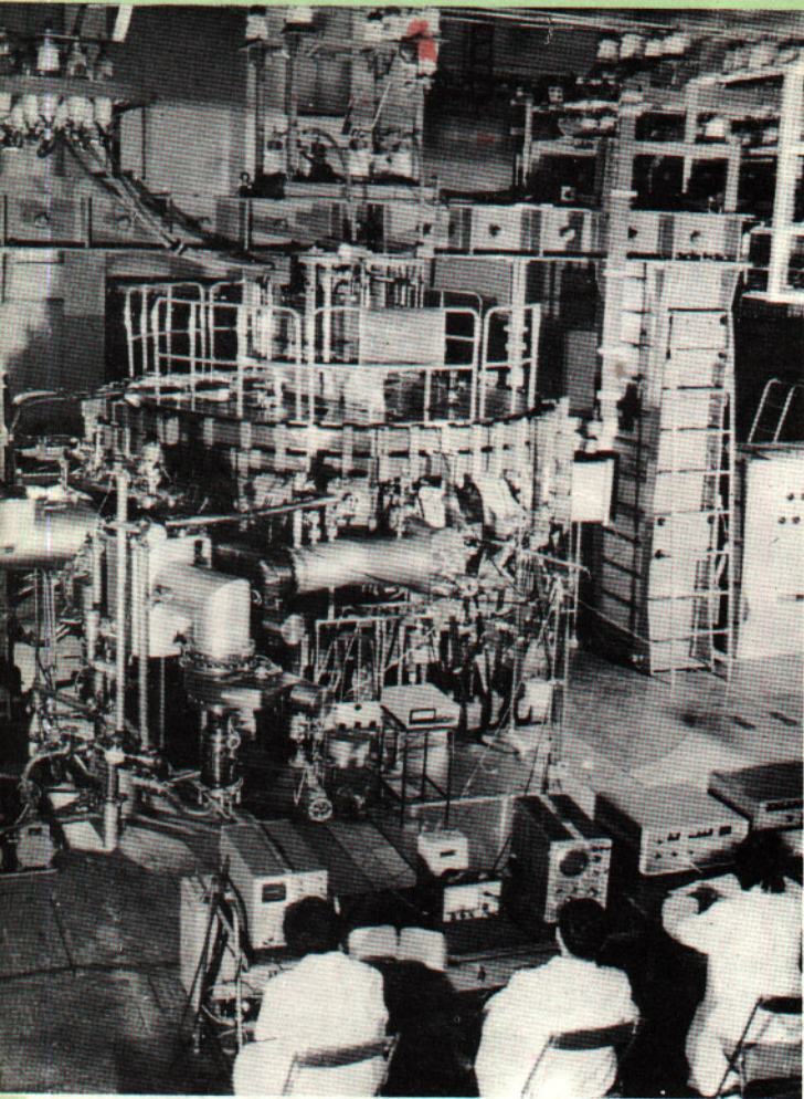
The heart of the controlled nuclear fusion experimental device.
