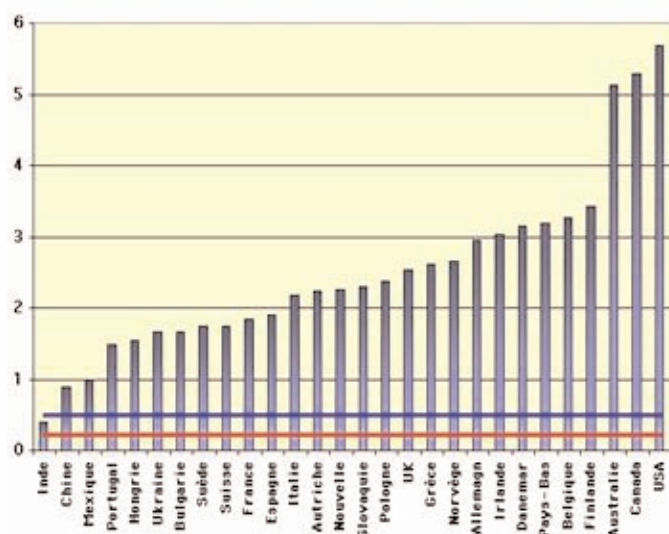
Fig. 4. Emissions of CO2 due to the combustion of fossil fuels (in tonnes of carbon) by person and by country (the other greenhouse gases are not taken into account) and level of stabilisation for a population of six billion human beings (0.5 tonnes of carbon/person and per year). Source : A. Berger, 2005.
