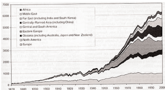
Fig. 1. Historic responsibility of groups of countries in climate change. Changes in volumes of carbon emitted from 1870 to 2000, by region of the world. The current volume of emissions is near to 8 gigatonnes of carbon per year (28.8 Gt of CO 2 ). Source: Oakridge National Laboratory.
