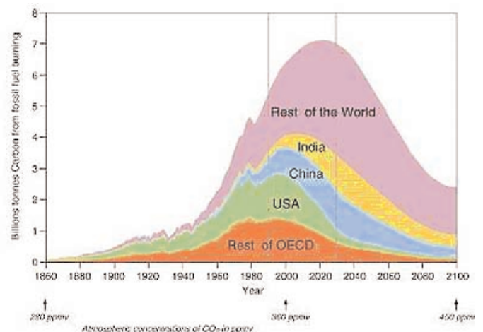
Figure 16. Illustrating the proposal "Contraction and Convergence", leading to stabilisation of atmospheric carbon dioxide at 450 ppm (from GCI)
